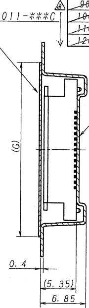
SECT. H-H
